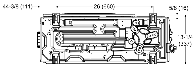
BOTTOM VIEW
